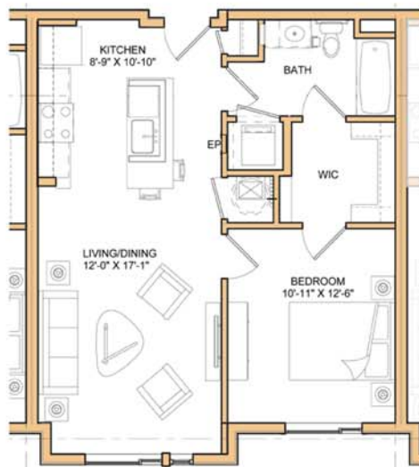
One Bedroom Unit Plan
