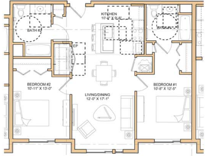
Two Bedroom Accessible Unit Plan
