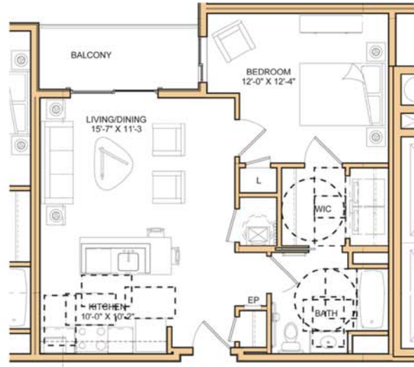
One Bedroom Accessible Unit Plan
