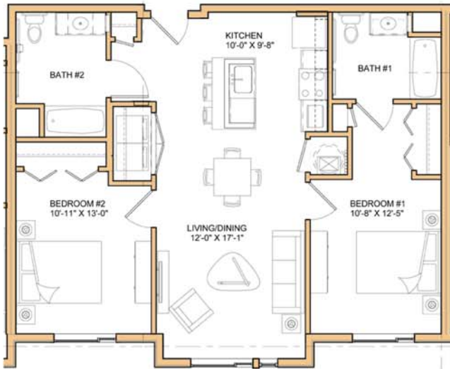
Two Bedroom Unit Plan
